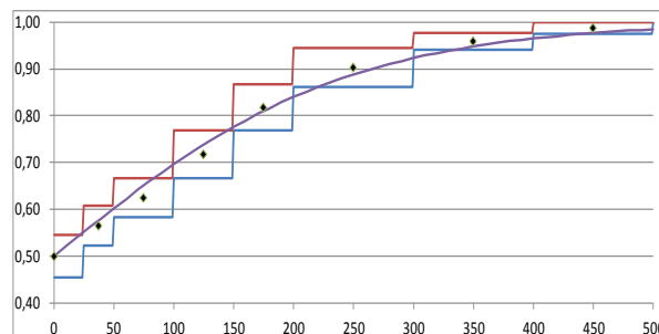
Fig. 1 Probabilities of average victories smoothed by Bradley-Terry model [3]
