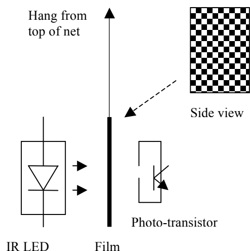
Fig. 4 Design of the optical displacement transducer
